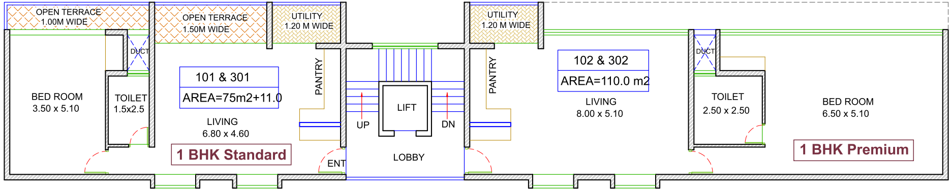
1ST FLOOR & 3RD FLOOR PLAN
